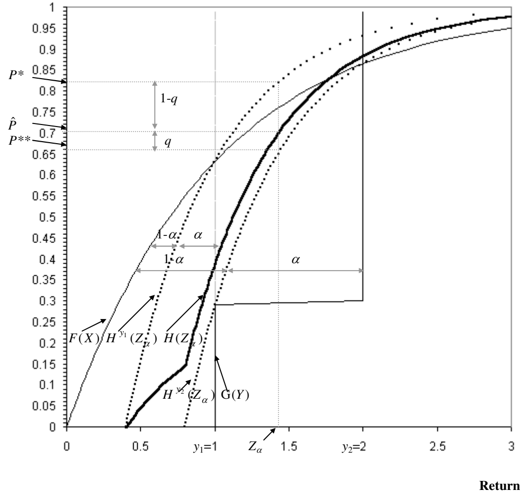
Figure 1. A graphical exposition of Proposition 1
